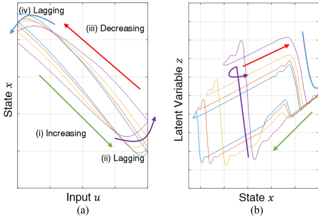
Fig. 13. (a) Hysteresis curve between input u and state x . (b) Temporal flows of one of the hidden variables z from the encoder part of the dynamics model p(x_{t+1} | x_t, u_{t-1}, u_t) .
