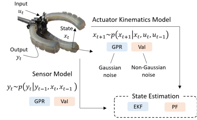
Fig. 1. Overall concept of probabilistic modeling and Bayesian filtering of soft robot. We use both models of actuator kinematics and sensor dynamics to improve the accuracy of the state estimation. The models are constructed to handle nonlinearity and temporal correlation of hysteresis in the sense of probabilistic data-driven function. We can handle both Gaussian and non-Gaussian noises using Gaussian process regression with extended Kalman filter, and variational inference with a particle filter, respectively.
