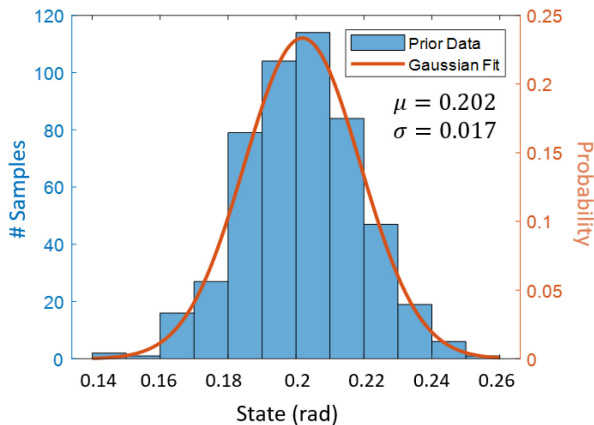
Fig. 11. Histogram of the sampled population of the variational inference in the dynamics model with the input signal from 20 s in Fig. 10(f).
