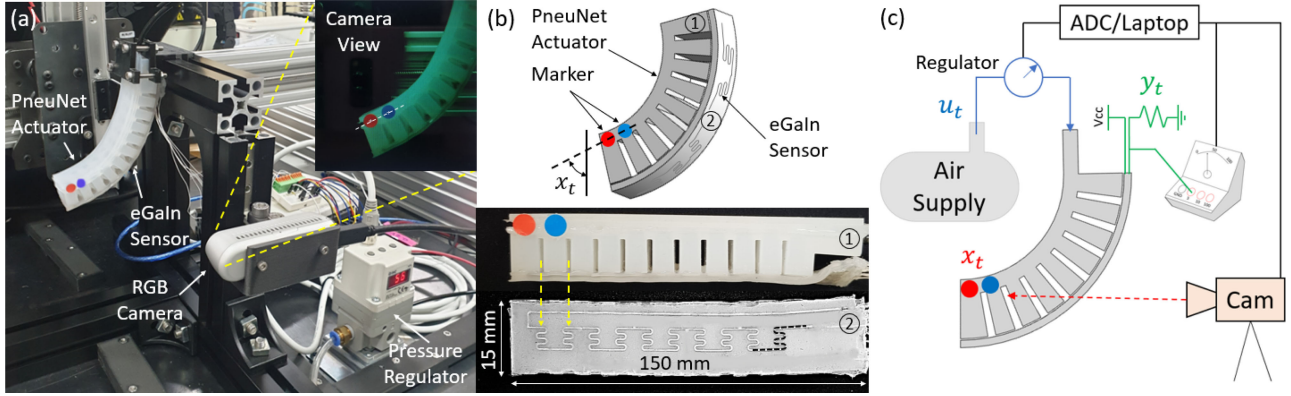
Fig. 7. (a) Experimental setup that consists of a pressure regulator, a PneuNet soft actuator with an embedded eGaIn soft sensor, and an RGB camera for tracking the motion of the actuator. The camera tracks the position of two markers to calculate the orientation. (b) Side and top views of the actuator with an embedded soft sensor. The camera collects the position of the markers and calculates the reference state x_t as an angle of the end-effector orientation relative to the vertical axis. The black dashed line in the bottom figure indicates the configuration of an eGaIn channel. The yellow dashed lines show the locations of the eGaIn channels aligned between air chambers. (c) Schematics of data acquisition setup for experiment. Compressed air is injected with predefined guide u_t , and the camera records the state x_t , and the voltmeter receives the sensor output y_t .
