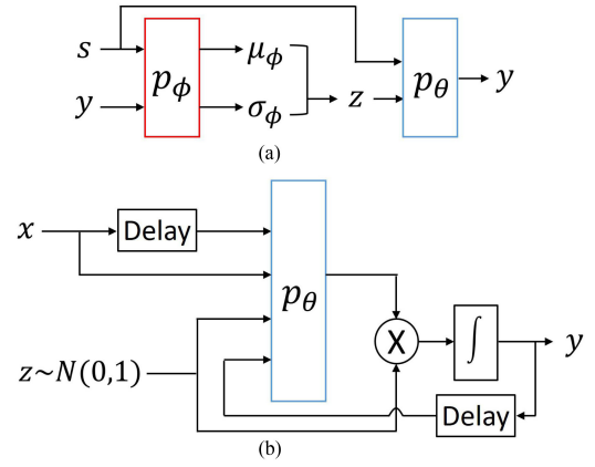
Fig. 6. (a) Given input s_t := [x_t, x_{t-1}, y_{t-1}]^\top and target y_t , encoder network parameterized by \phi and decoder network parameterized by \theta can be trained by maximizing ELBO equation. (b) In real-time testing, encoder network is removed and latent feature z is replaced by a predefined distribution.
