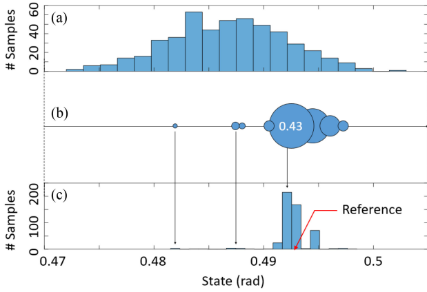
Fig. 12. Resampling procedure of PF with testing signal from 35.5 s in Fig. 10(f). (a) Result of the generative network of the dynamics model ( B_t in Algorithm 1) in histogram. (b) Corresponding likelihood of the sensor model ( W_t in Algorithm 1). (c) Resampling result in histogram.
