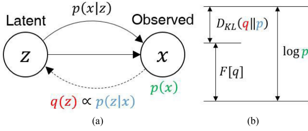
Fig. 2. (a) Latent variable model that consists of latent variable z , observable x , connected with encoder p(z|x) and decoder p(x|z) . (b) To maximize the posterior, both KL divergence and variational free energy F[q] are considered.
